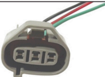
Fuel Pump Maximo/M&M
