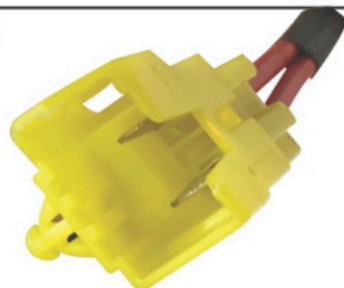
Single Fuse Holder MAXI Fuse
