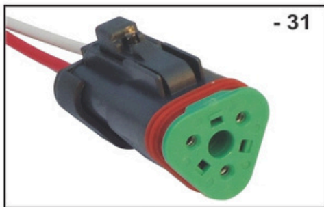
3 Pole JCB/Ashok Leyland
